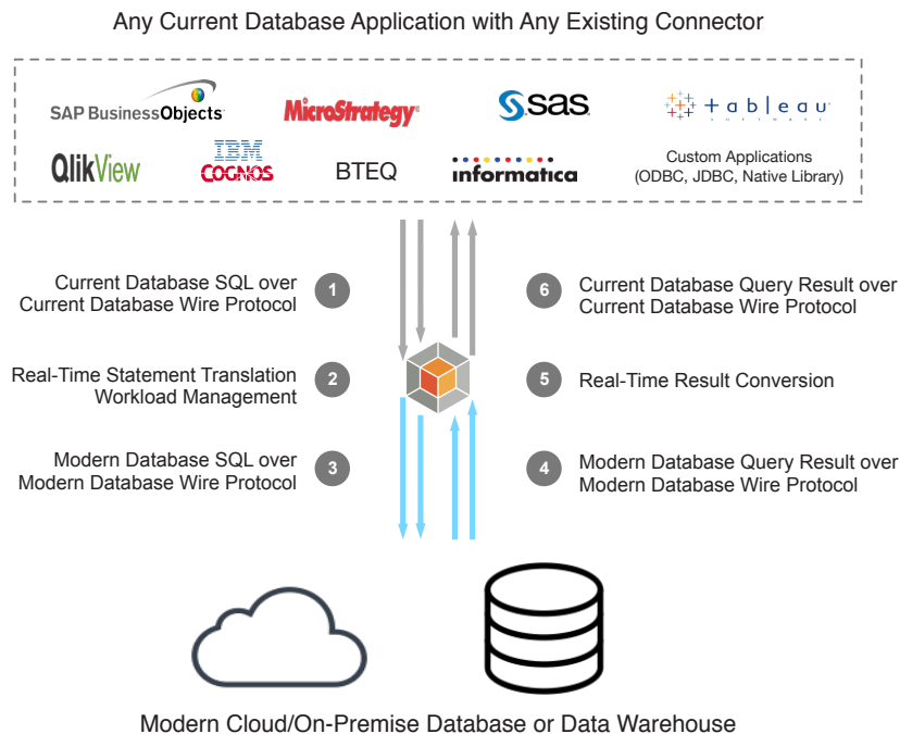
Figure 1: Enabling Legacy Applications for Any Cloud or On-Premise Database
